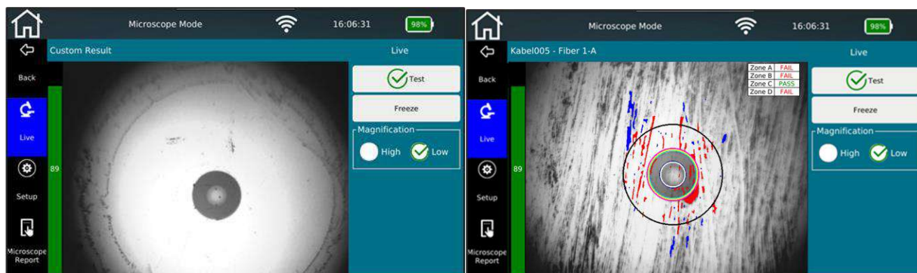
Figure 57 – Individual Mikroscope test
