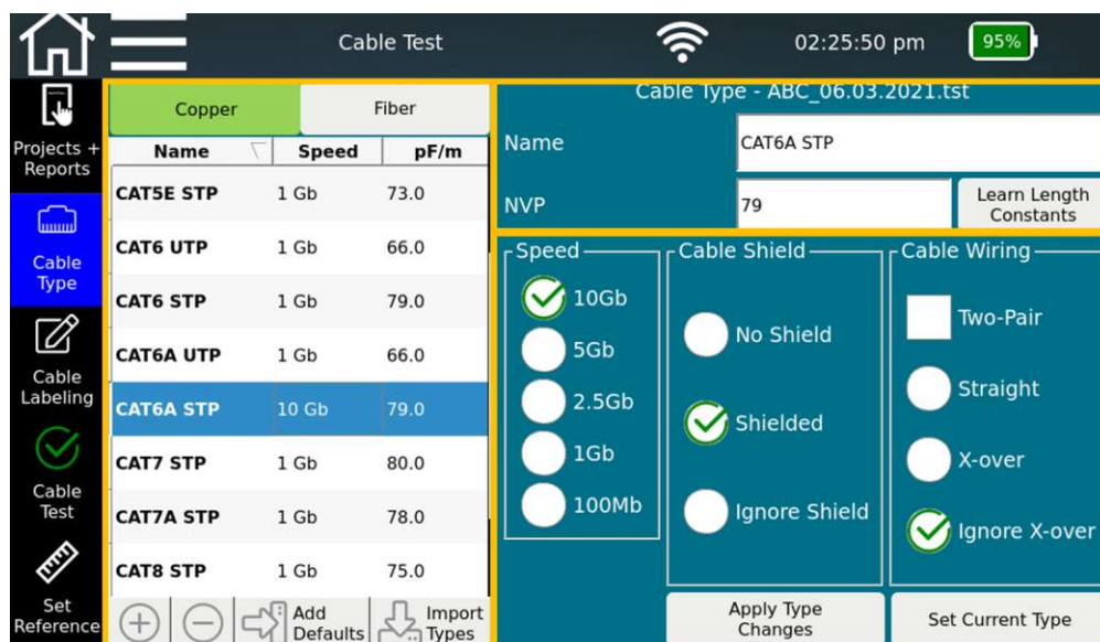
Figure 28 - Cable types and test parameters - Cu
