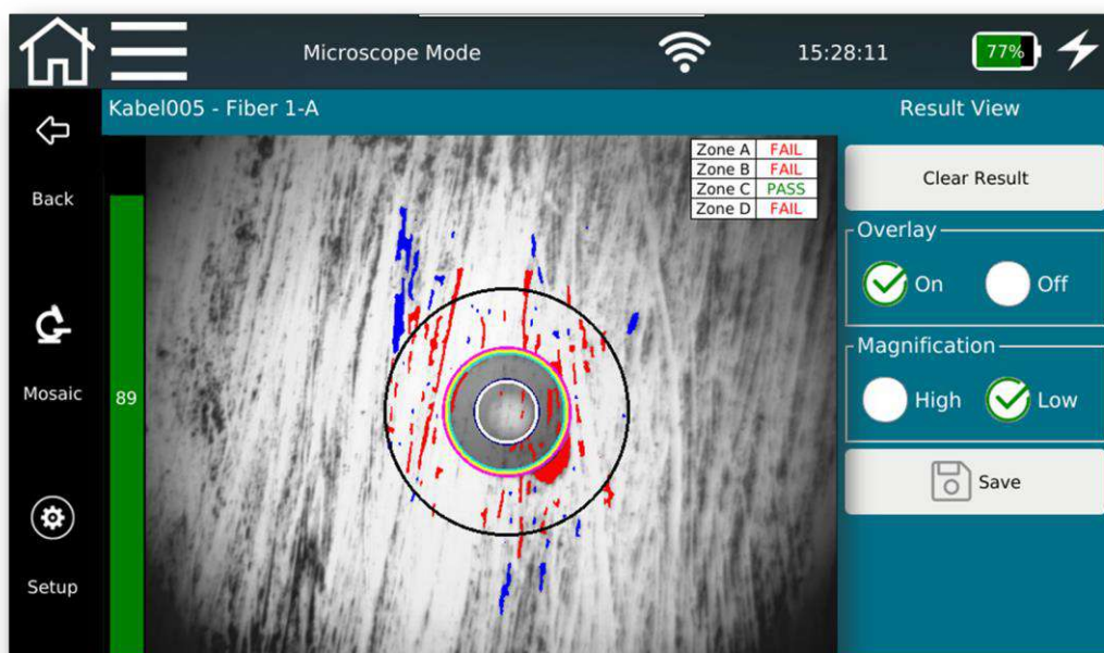
Figure 37 — Result view of a failed microscope test of a connector end face
