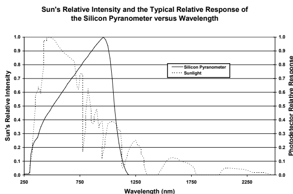
Plot A: S-LIB-M003 Silicon Pyranometer Response Curve
