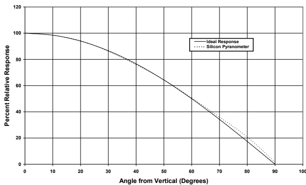
Plot B: S-LIB-M003 Typical Cosine Response Curve
